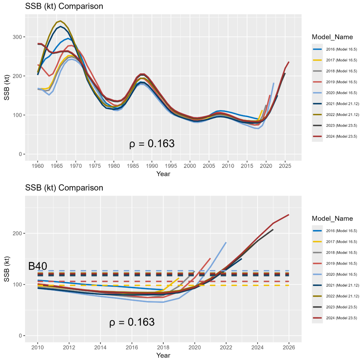
Figure 3.48. Results of the ‘all model’ historical retrospective illustrating estimated and projected (terminal year + 2 years) spawning stock biomass (in kilotons). Results are based on the accepted model in each terminal model year, including application of the 23.5 model for 2023 and 2024, the 21.12 model for the 2021 and 2022 model years, and the 16.5 model for earlier model years. The top panel shows the entire time series of SSB from each assessment model, while the bottom panel shows the same results since 2010 overlaid with corresponding estimates of B_{40\%} . Mohn’s rho for two year SSB projections is provided below the lines in each plot.
