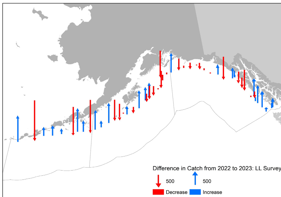
Figure 3.5. Comparison of the 2022 and 2023 longline survey in the Gulf of Alaska in terms of the difference in numbers of fish caught per station from 2022 in the 2023 survey. Numbers are not corrected for sperm whale depredation.
