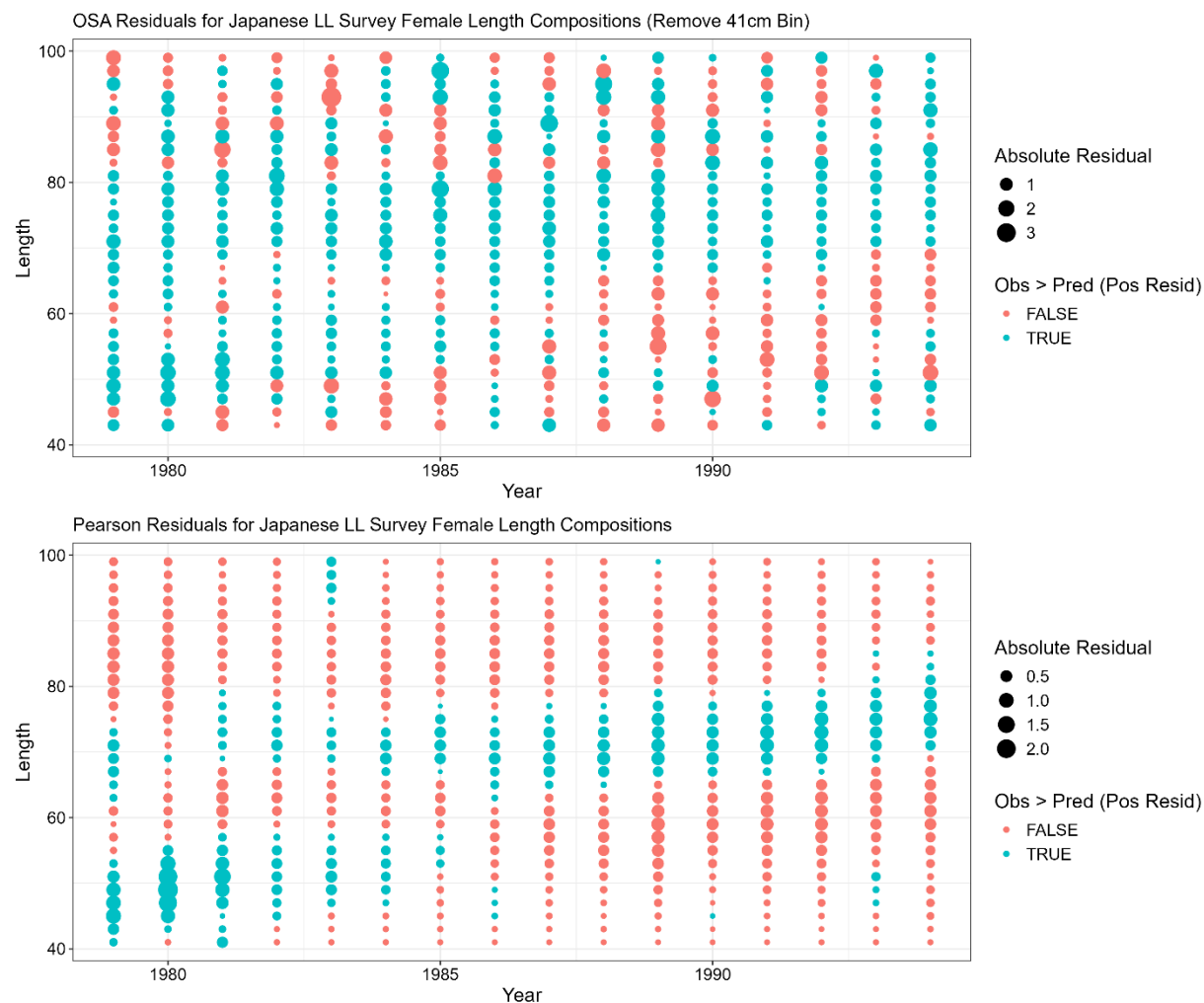
Figure 3C.5. Japanese cooperative longline survey female length composition one step ahead (OSA; top row) and Pearson residuals (bottom row). Color denotes negative (red) or positive (blue) residuals. For OSA residuals the first size class was removed.
