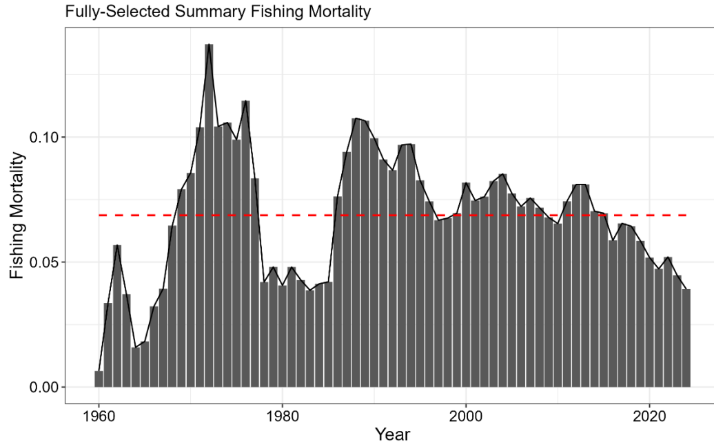
Figure 3.42. Time series of fully selected fishing mortality aggregated across the fixed gear and trawl fisheries. Red line is the mean fishing mortality for the entire time series.
