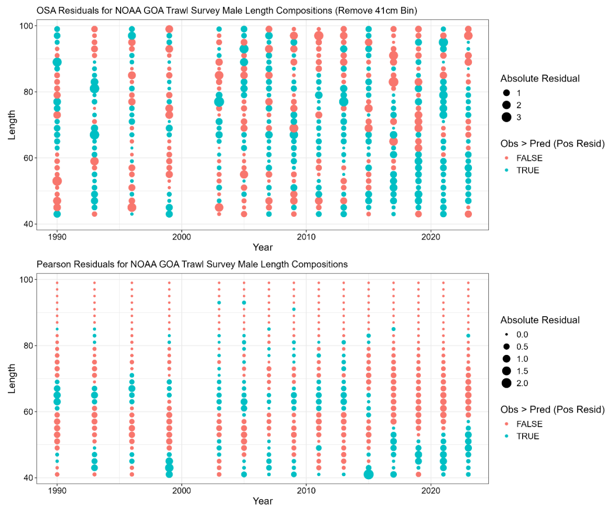
Figure 3C.8. NOAA Gulf of Alaska trawl survey male length composition one step ahead (OSA; top row) and Pearson residuals (bottom row). Color denotes negative (red) or positive (blue) residuals. For OSA residuals the first size class was removed.
