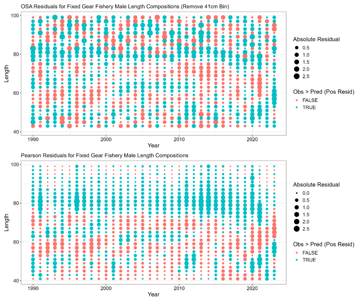
Figure 3C.10. Domestic fixed gear fishery male length composition one step ahead (OSA; top row) and Pearson residuals (bottom row). Color denotes negative (red) or positive (blue) residuals. For OSA residuals the first size class was removed.
