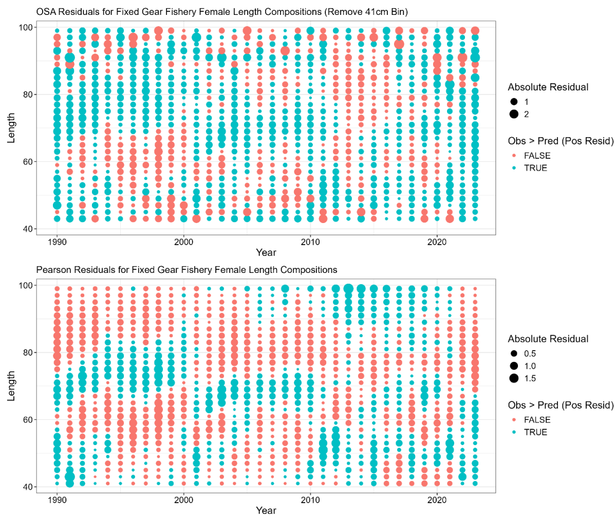
Figure 3C.11. Domestic fixed gear fishery female length composition one step ahead (OSA; top row) and Pearson residuals (bottom row). Color denotes negative (red) or positive (blue) residuals. For OSA residuals the first size class was removed.
