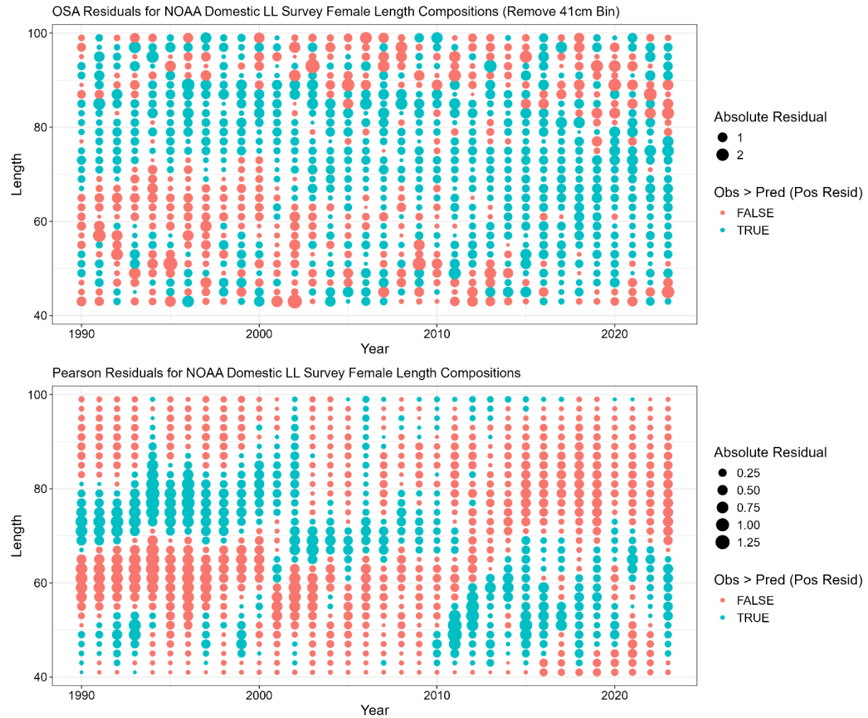
Figure 3C.7. NOAA domestic longline survey female length composition one step ahead (OSA; top row) and Pearson residuals (bottom row). Color denotes negative (red) or positive (blue) residuals. For OSA residuals the first size class was removed.
