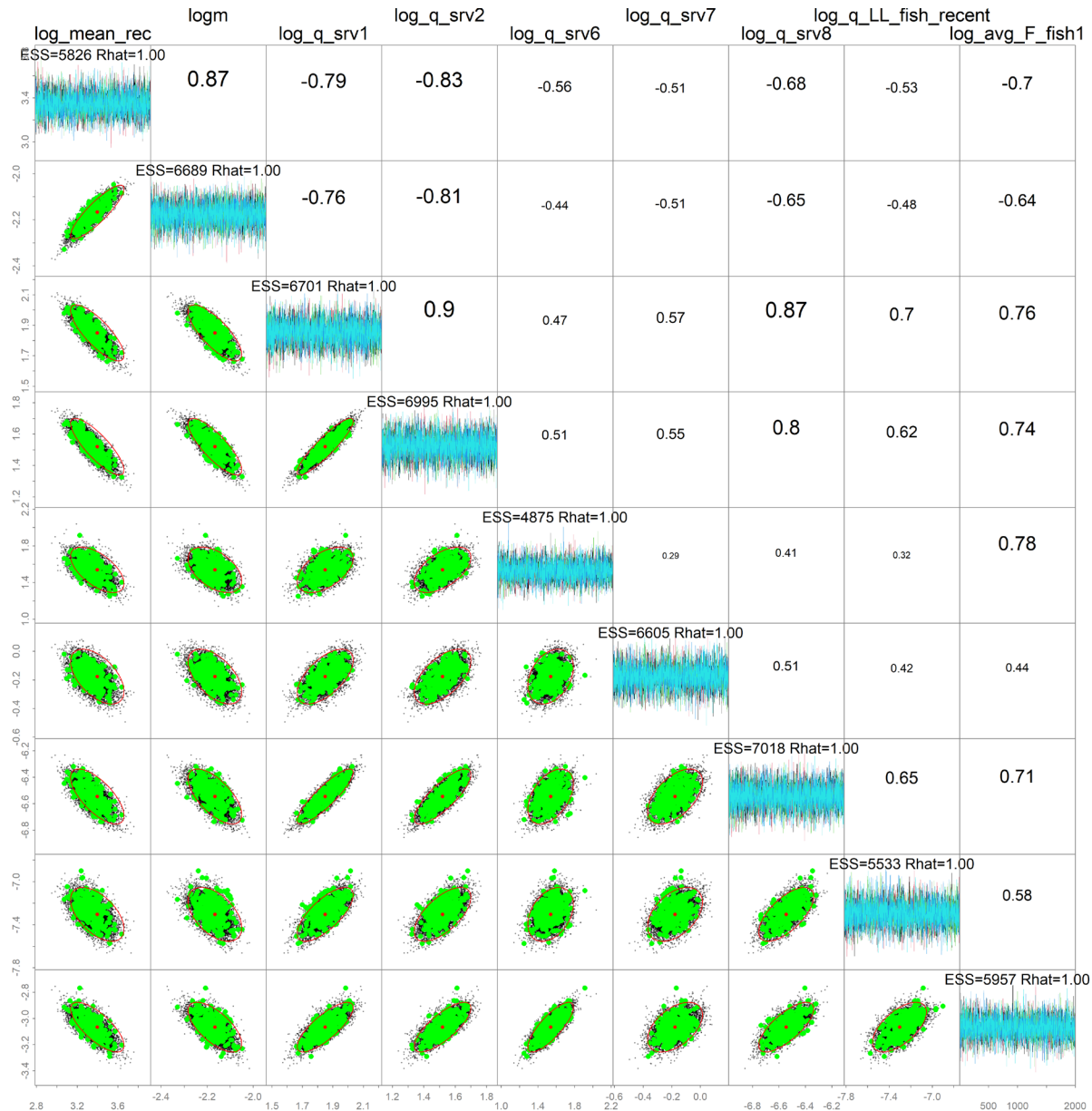
Figure 3C.14. MCMC pairwise correlation plots among key model parameters, where diagnostics are shown along the diagonal and parameter correlations are shown in the upper right quadrant.
