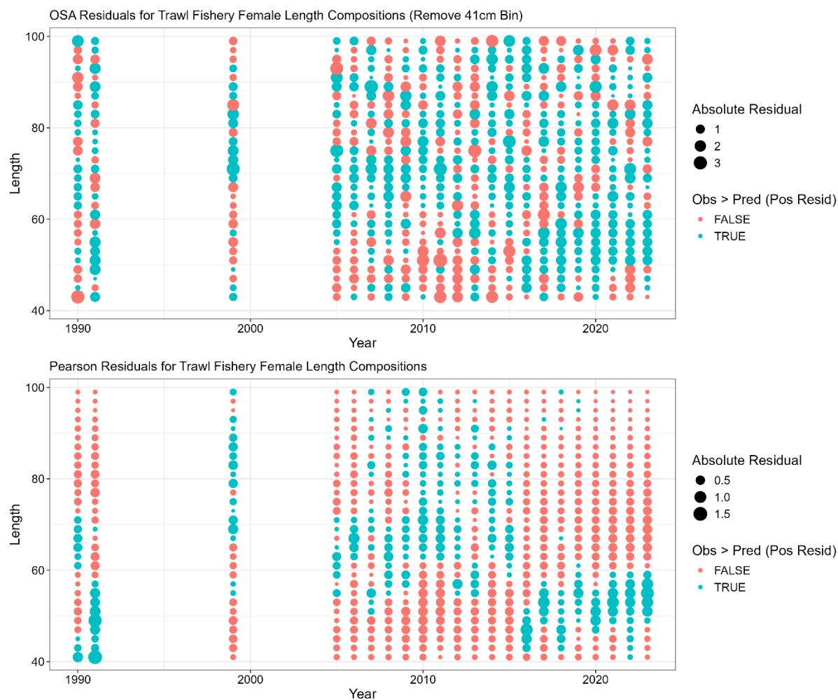
Figure 3C.13. Domestic trawl gear fishery female length composition one step ahead (OSA; top row) and Pearson residuals (bottom row). Color denotes negative (red) or positive (blue) residuals. For OSA residuals the first size class was removed.
