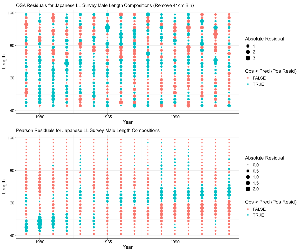
Figure 3C.4. Japanese cooperative longline survey male length composition one step ahead (OSA; top row) and Pearson residuals (bottom row). Color denotes negative (red) or positive (blue) residuals. For OSA residuals the first size class was removed.
