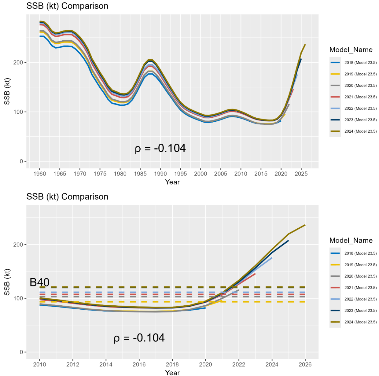
Figure 3.49. Results of the ‘current model’ historical retrospective illustrating estimated and projected (terminal year + 2 years) spawning stock biomass (in kilotons). Results are based on application of the 23.5 model to the available data at the time of previous sablefish assessments. The top panel shows the entire time series of SSB from each assessment model, while the bottom panel shows the same results since 2010 overlaid with corresponding estimates of B_{40\%} . Mohn’s rho for two year SSB projections is provided below the lines in each plot.
