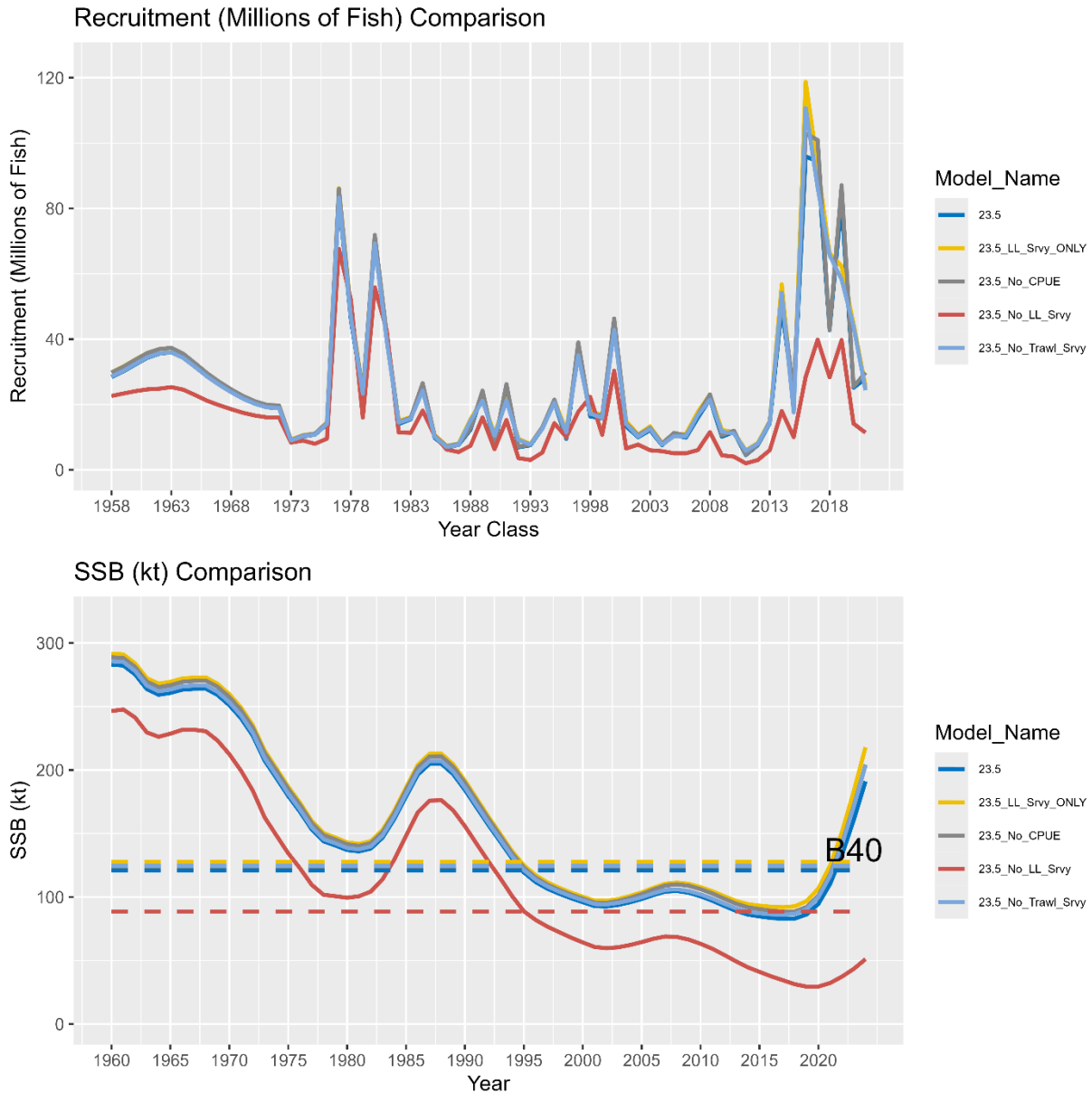
Figure 3.52. Results of an index sensitivity analysis where the model is rerun after removing each index (and any associated compositional data in the case of fishery independent surveys) one at a time. The top panel illustrates the model estimated recruitment (millions of fish). The bottom panel depicts the time series of SSB (kt).
