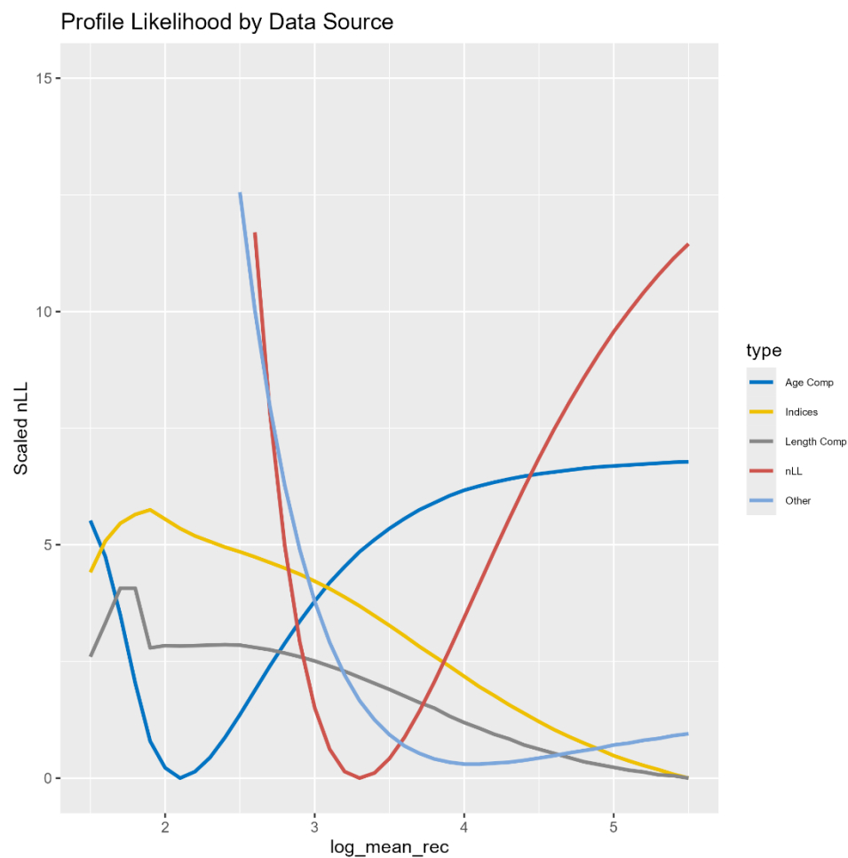
Figure 3.50. Likelihood profiles by data type (line color) for the mean recruitment parameter in logarithmic space.
