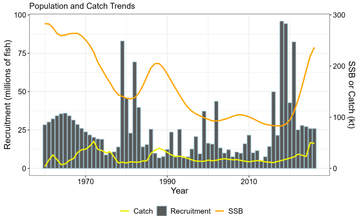
Figure 3.55. Time series of sablefish SSB (orange line), catch (yellow line), and recruitment (grey bars). Projected dynamics for 2025 and 2026 are included based on the maximum permissible ABC and average recruitment. Note the cyclical dynamics associated with spasmodic recruitment. Transitory increases in SSB subsequent to periods of strong recruitment are often followed by a persistent downward time series trend. Catches often rapidly increase following high recruitment periods, while recruitment reverts back towards average levels.
