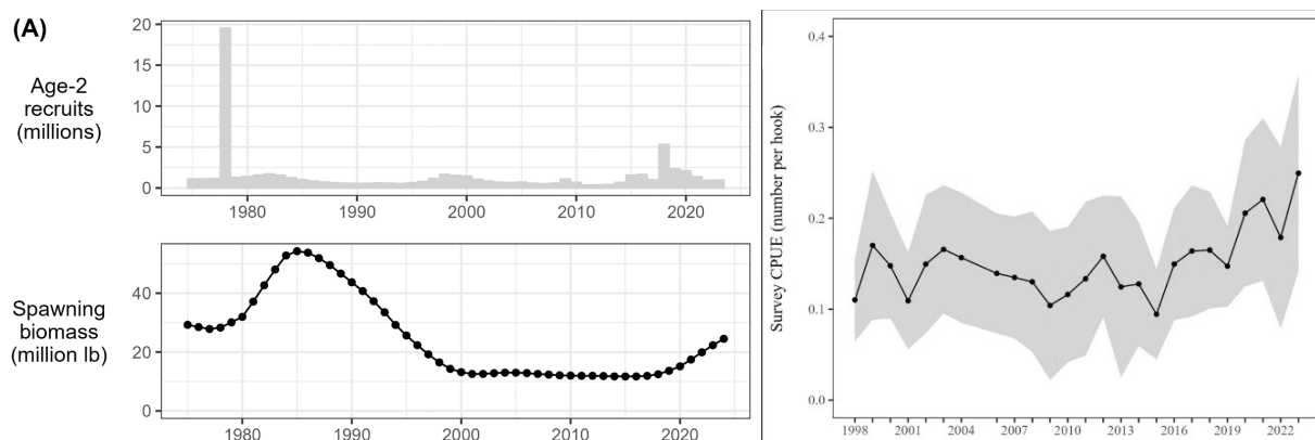
Figure 3.8a. Model predictions for the ADFG Northern Southeast Inside (NSEI) sablefish stock assessment (left panels; reproduced here with permission from Rhea Ehresmann, pers. comm., https://github.com/commfish/seak_sablefish ) of age-2 recruitment (millions; top) and female spawning stock biomass (million pounds; bottom). Southern Southeast Inside (SSEI) sablefish longline survey catch-per-unit-effort (CPUE) in individuals per hook (right panel) from 1998 to 2023 (except 2005; reproduced here with permission from Rhea Ehresmann, pers. Comm.).
