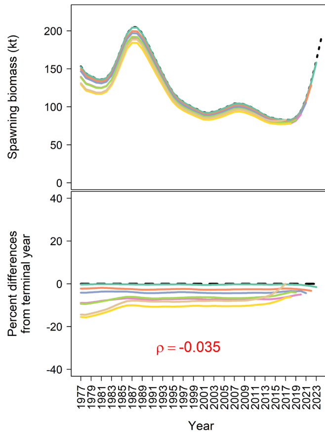
Figure 3.46. Retrospective trends for spawning biomass (top) and percent difference from terminal year (bottom). Mohn's rho ( \rho ) is provided in red (bottom panel).
