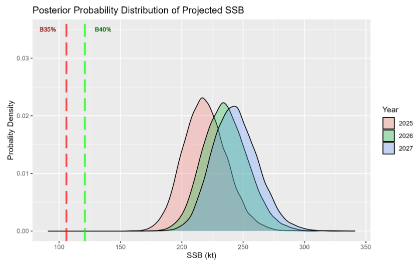
Figure 3.45. Posterior probability distribution from MCMC for projected spawning biomass (kilotons) in years 2025 – 2027. The dashed lines are B_{35\%} and B_{40\%} .
