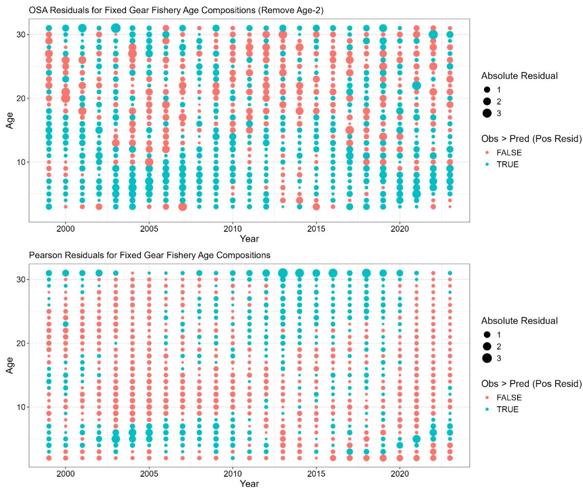
Figure 3C.3. Domestic fixed gear fishery age composition one step ahead (OSA; top row) and Pearson residuals (bottom row). Color denotes negative (red) or positive (blue) residuals. For OSA residuals the first age class was removed.
