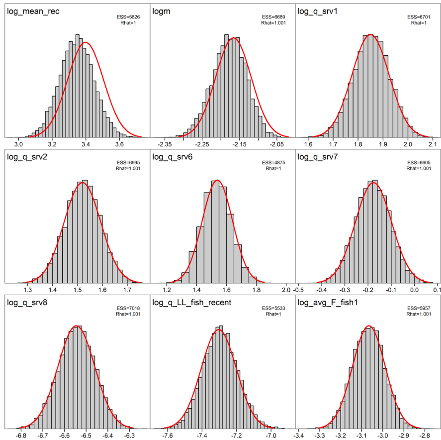
Figure 3.44. Key parameter marginal posterior histograms from MCMC and asymptotic normal distributions (red line) from the inverse Hessian (MLE). MCMC effective sample size (ESS) and R-hat estimates are printed in the top right corner.
