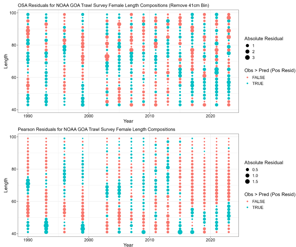
Figure 3C.9. NOAA Gulf of Alaska trawl survey female length composition one step ahead (OSA; top row) and Pearson residuals (bottom row). Color denotes negative (red) or positive (blue) residuals. For OSA residuals the first size class was removed.
