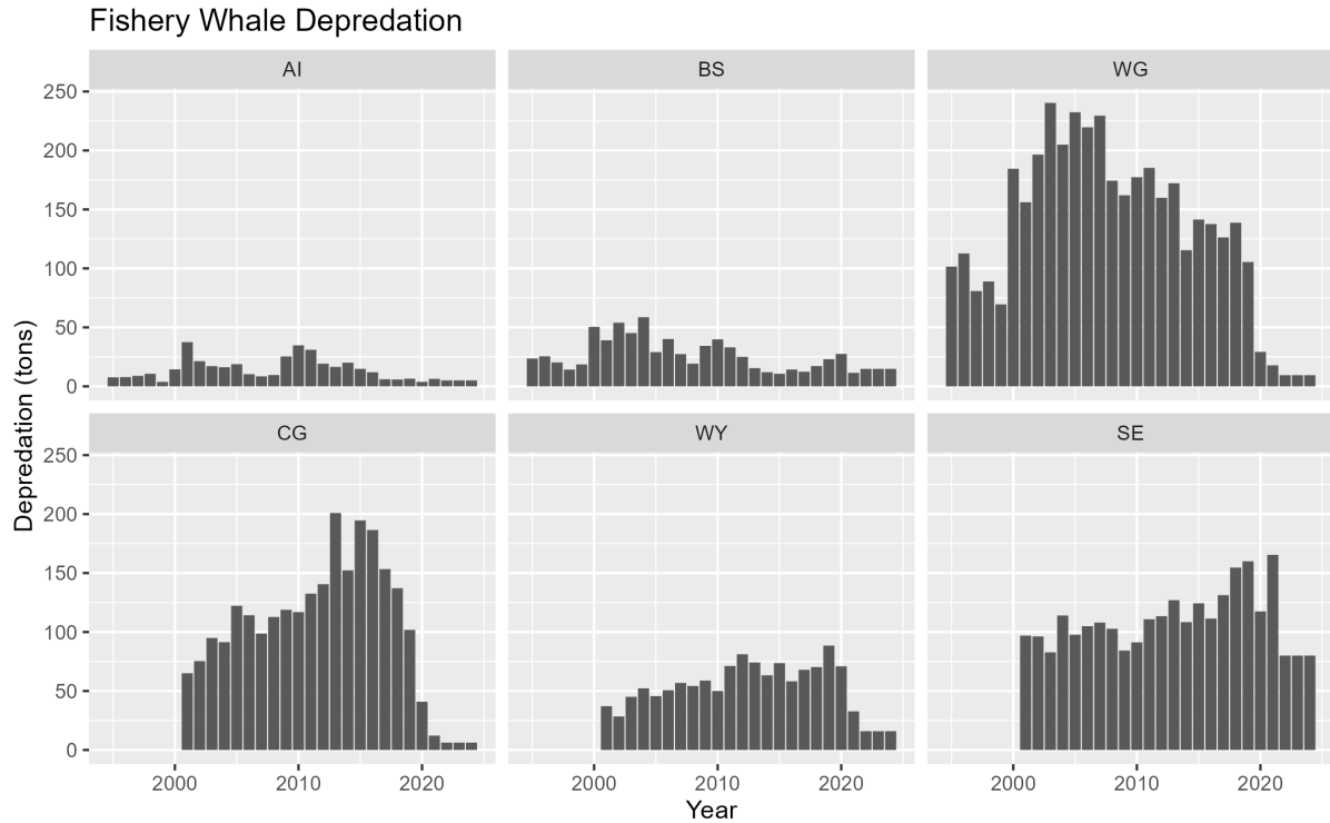
Figure 3.7. Estimated whale depredation in the sablefish fixed gear fishery. Depredation estimates reflect catch removals (tons) by region (panel) due to orcas (top row) and sperm whales (bottom row). Starting in 2023 estimates were held constant at 2022 values.
