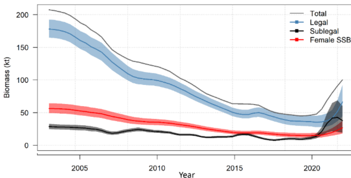
Figure 3.8b. Time series of total biomass, legal-sized biomass, sub-legal-sized biomass, and female spawning biomass (SSB) estimates for the British Columbia stock of sablefish based on weighted averages over the five OM scenarios used in 2022. Note that total, legal, and sub-legal biomass estimates include both female and male fish, while SSB is shown for only female Sablefish (reproduced here with permission from Kendra Holt, DFO Canada, pers. comm.).
