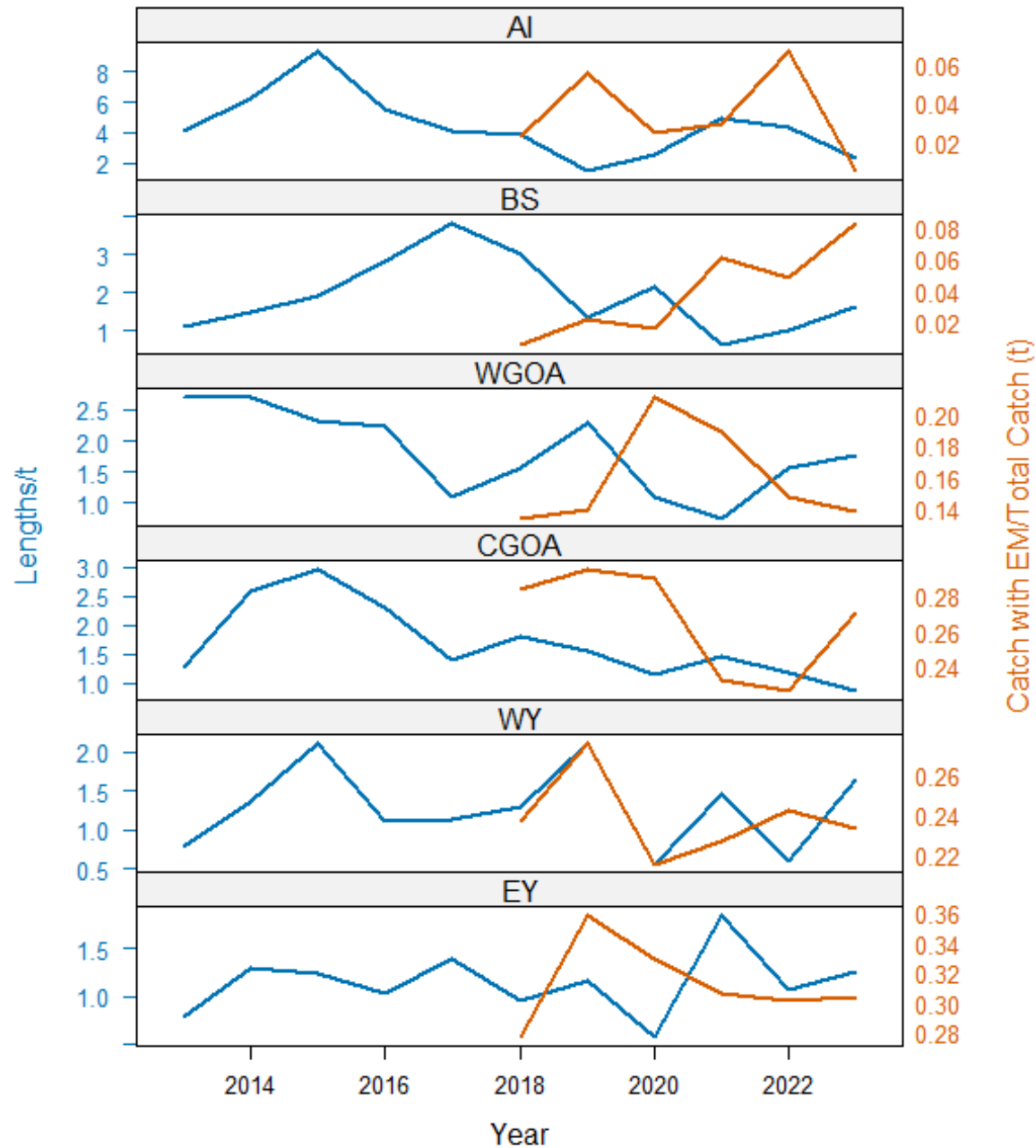
Figure 3.F.13. The proportion of fixed gear (pot and hook and line gear) sablefish catch from vessels using electronic monitoring (EM strata catch in t/total fixed gear catch in t) and the rate of sablefish length sampling (lengths per t) of sablefish catch from fixed-gear vessels. Areas include the Aleutian Islands (AI), Bering Sea (BS), Western Gulf of Alaska (WGOA), Central Gulf of Alaska (CGOA), West Yakutat (WY), and East Yakutat (EY)
