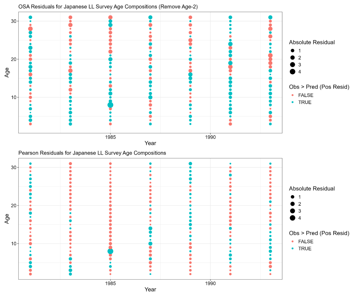
Figure 3C.1. Japanese cooperative longline survey age composition one step ahead (OSA; top row) and Pearson residuals (bottom row). Color denotes negative (red) or positive (blue) residuals. For OSA residuals the first age class was removed.
