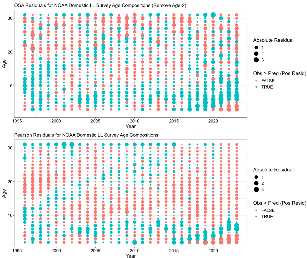
Figure 3C.2. NOAA domestic longline survey age composition one step ahead (OSA; top row) and Pearson residuals (bottom row). Color denotes negative (red) or positive (blue) residuals. For OSA residuals the first age class was removed.
