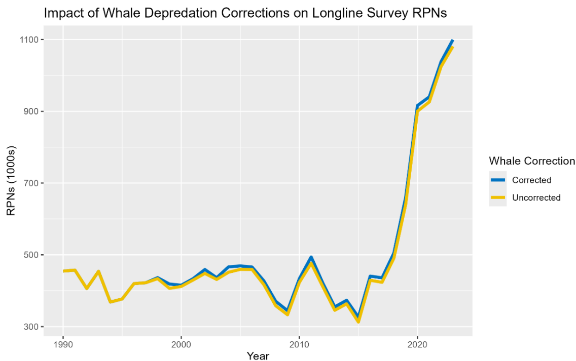
Figure 3.6. Longline survey relative population numbers (1000s of fish) with (blue line) and without (yellow line) corrections for sperm whale depredation. Note that these values do not include interpolations for areas not surveyed in the given year (i.e., RPNs are less than the final index by the associated RPN in either the BS or AI, depending on which area was not surveyed).
