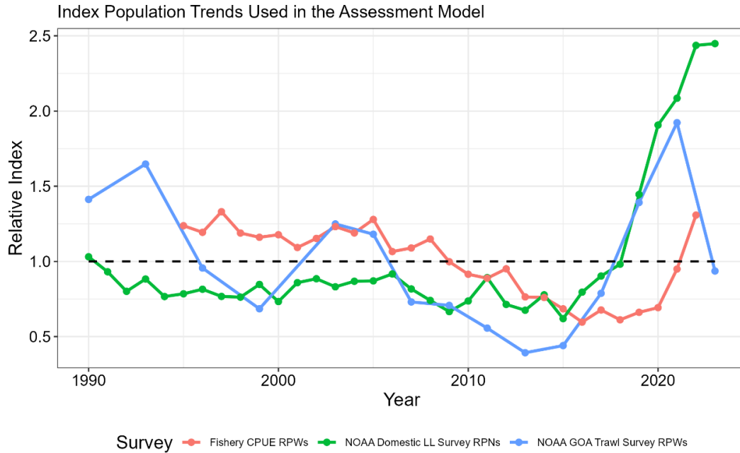
Figure 3.3. Comparison of the three indices used in the stock assessment model, including the NOAA domestic longline survey relative population numbers (RPNs), the fixed gear fishery standardized CPUE (in weight), and the NOAA Gulf of Alaska (stations < 500m depth) trawl survey relative population weights (RPWs). Each index is relativized to the associated mean value for the time series.
