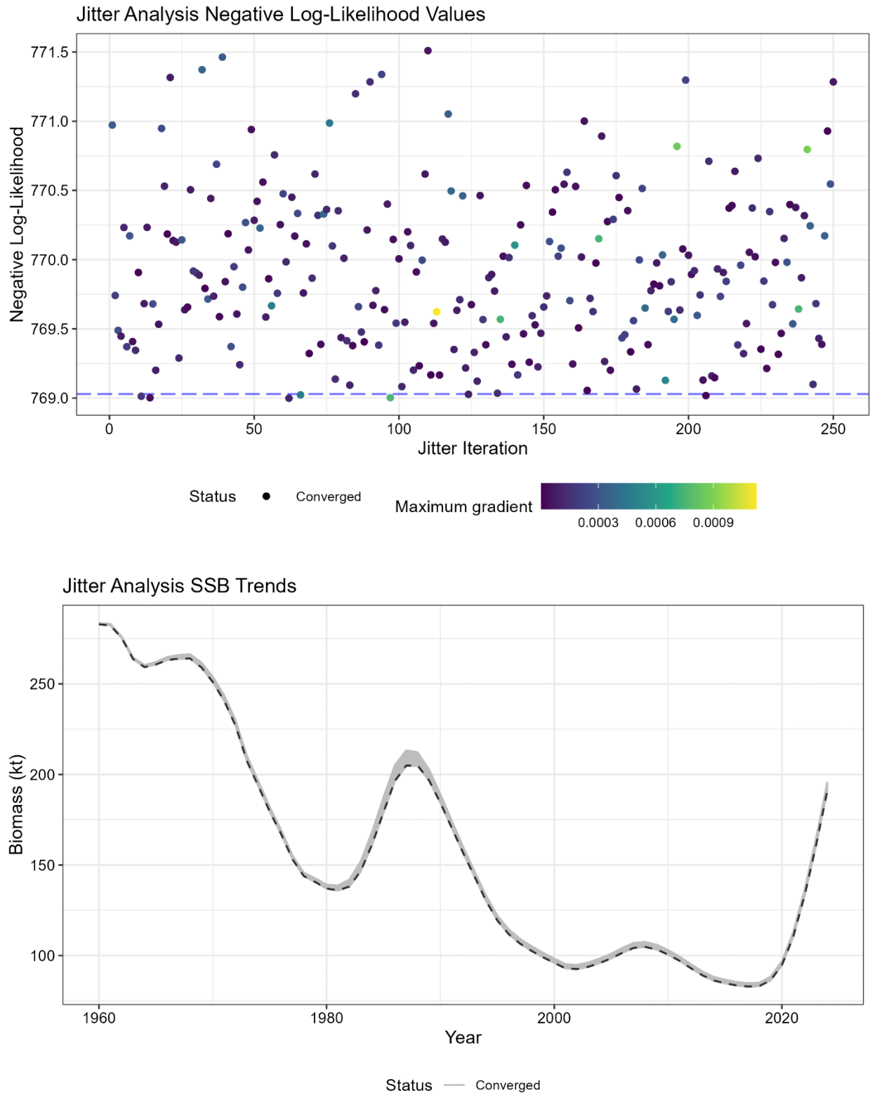
Figure 3.10. Results of the jitter analysis in terms of total negative log-likelihood (nll) values (top panel) and SSB estimates (kt; bottom panel). All 250 model runs are shown and the model with the smallest nll was used as the base model.
