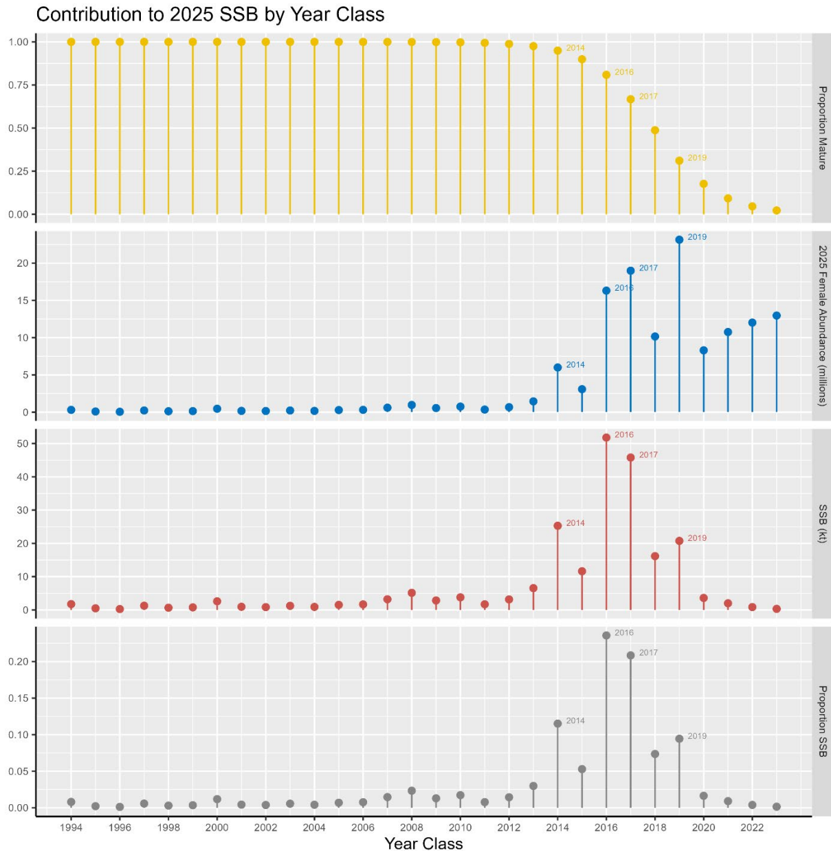
Figure 3.54. Proportion mature (top panel), projected 2025 female (assuming a 50:50 sex ratio) abundance (millions of fish; second panel from top), projected 2025 spawning stock biomass (kilotons; third panel from top), and proportional contribution to 2025 SSB (bottom panel) for each of the last 30 year classes. Note that the 1994 year class represents all contributions from all earlier year classes (i.e., fish in the plus group age). Abundance of the 2022 and 2023 year classes are based on mean recruitment, because these year classes have not yet been estimated in the 2024 assessment model.
