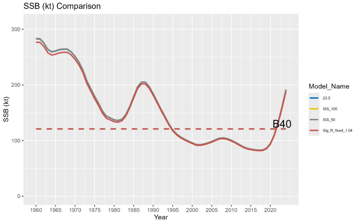
Figure 3.53. Results of the sensitivity runs for SSB in kt, where model naming conventions can be found in the main text.
